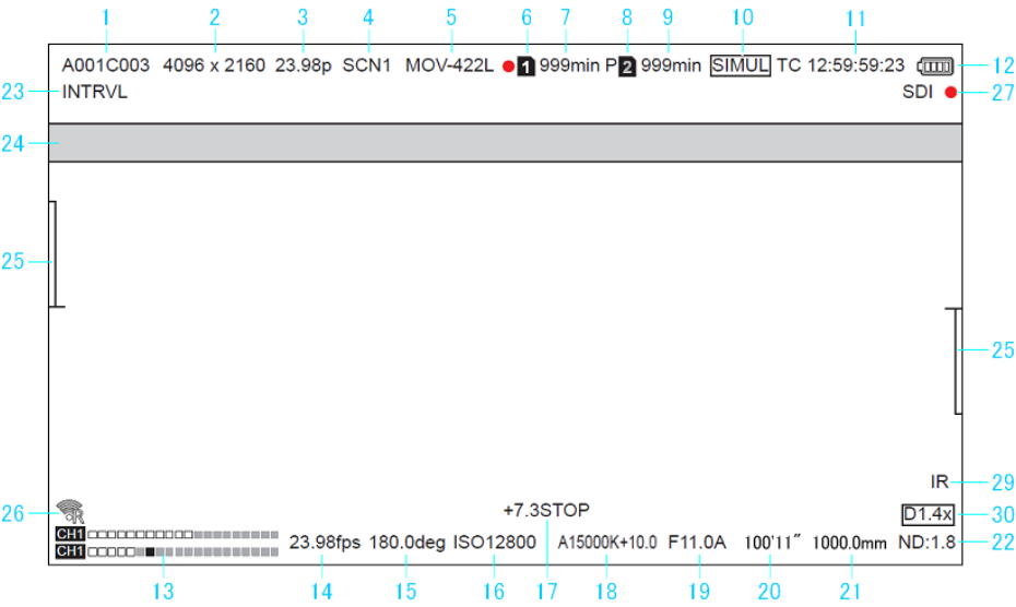
Camera status information display on the LCD monitor
